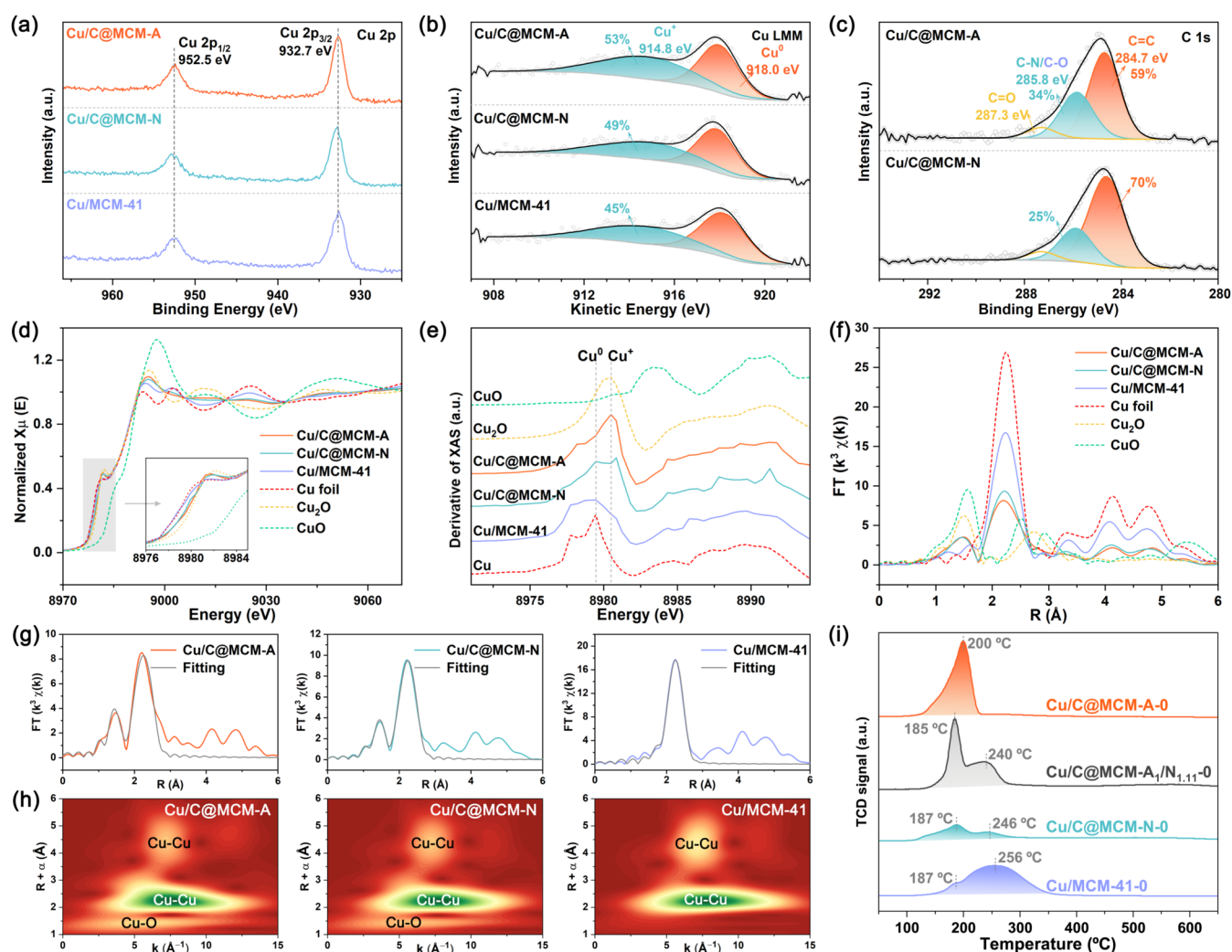
Figure 3. (a) High-resolution XPS spectra of Cu 2p and (b) in situ Cu LMM Auger spectra for the Cu/C@MCM-A, Cu/C@MCM-N, and Cu/MCM-41 catalysts. (c) XPS spectra of C 1s for Cu/C@MCM-A and Cu/C@MCM-N. (d) Normalized Cu K-edge XANES spectra, (e) first derivative of Cu K-edge XANES spectra, and (f) FT-EXAFS spectra at Cu K-edge for Cu/C@MCM-A, Cu/C@MCM-N, Cu/MCM-41, CuO, Cu 2 O, and Cu foil. (g) Fitting curves of FT-EXAFS spectra and (h) WT-EXAFS spectra for Cu/C@MCM-A, Cu/C@MCM-N, and Cu/MCM-41. (i) H 2 -TPR profiles of as-prepared Cu/C@MCM-A-0, Cu/C@MCM-A 1 /N 1,11 -0, Cu/C@MCM-N-0, and Cu/MCM-41-0.
